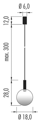
TECHNICAL DRAWING
