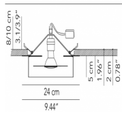
Recessed spotlight
