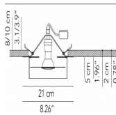
Recessed spotlight
