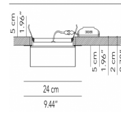
Recessed spotlight LED
